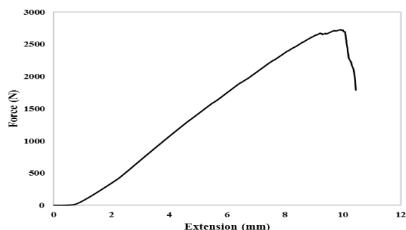
Fig. 6. Bending curve for GE (0) after aging.
