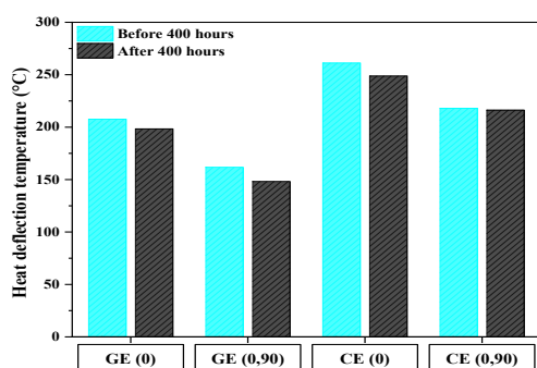
Fig. 8. The results of the HDT test for each sample before and after 400 hours of aging.
