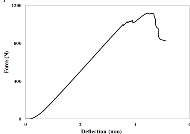
Fig. 5. Bending curve for CE (0) after aging.
