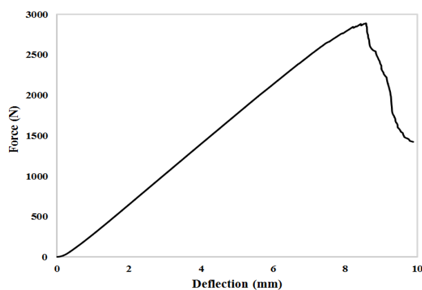
Fig. 4. Bending curve for GE sample with lamination (0).
