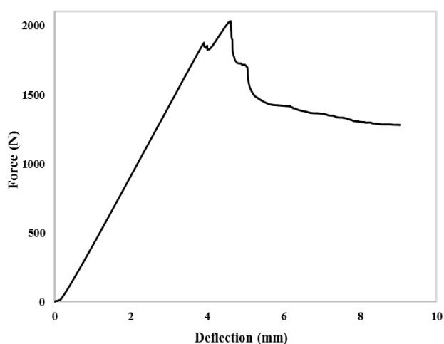
Fig. 3. Bending curve for CE sample with lamination (0).
