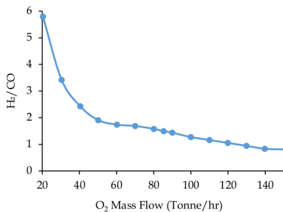
Fig. 3. Effect of Increased Oxygen Input on the H 2 /CO Ratio in the Gasifier Outlet.
