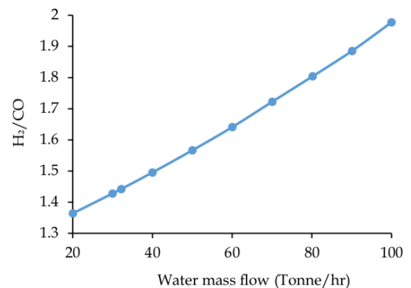
Fig. 4. Effect of Increased Water Input on the H 2 /CO Ratio in the Gasifier Outlet.
