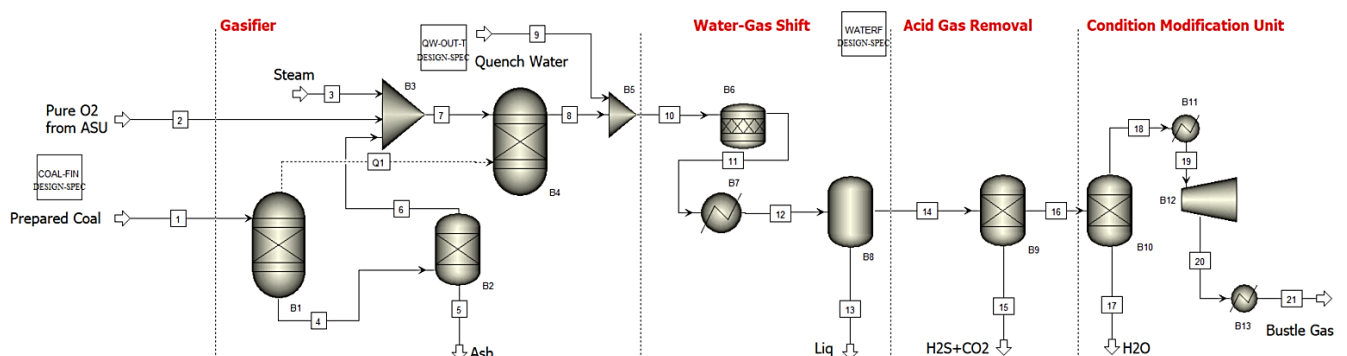
Fig. 2. PFD of the Gasification Unit.
