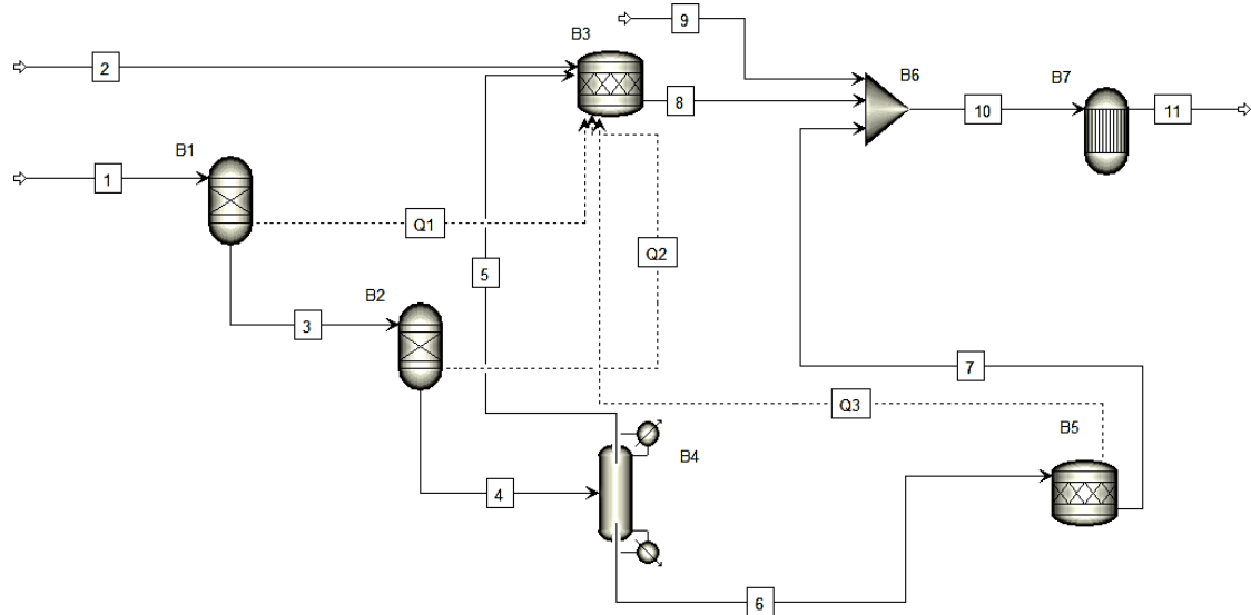
Fig. 1. Base Simulation Flow Sheet.
